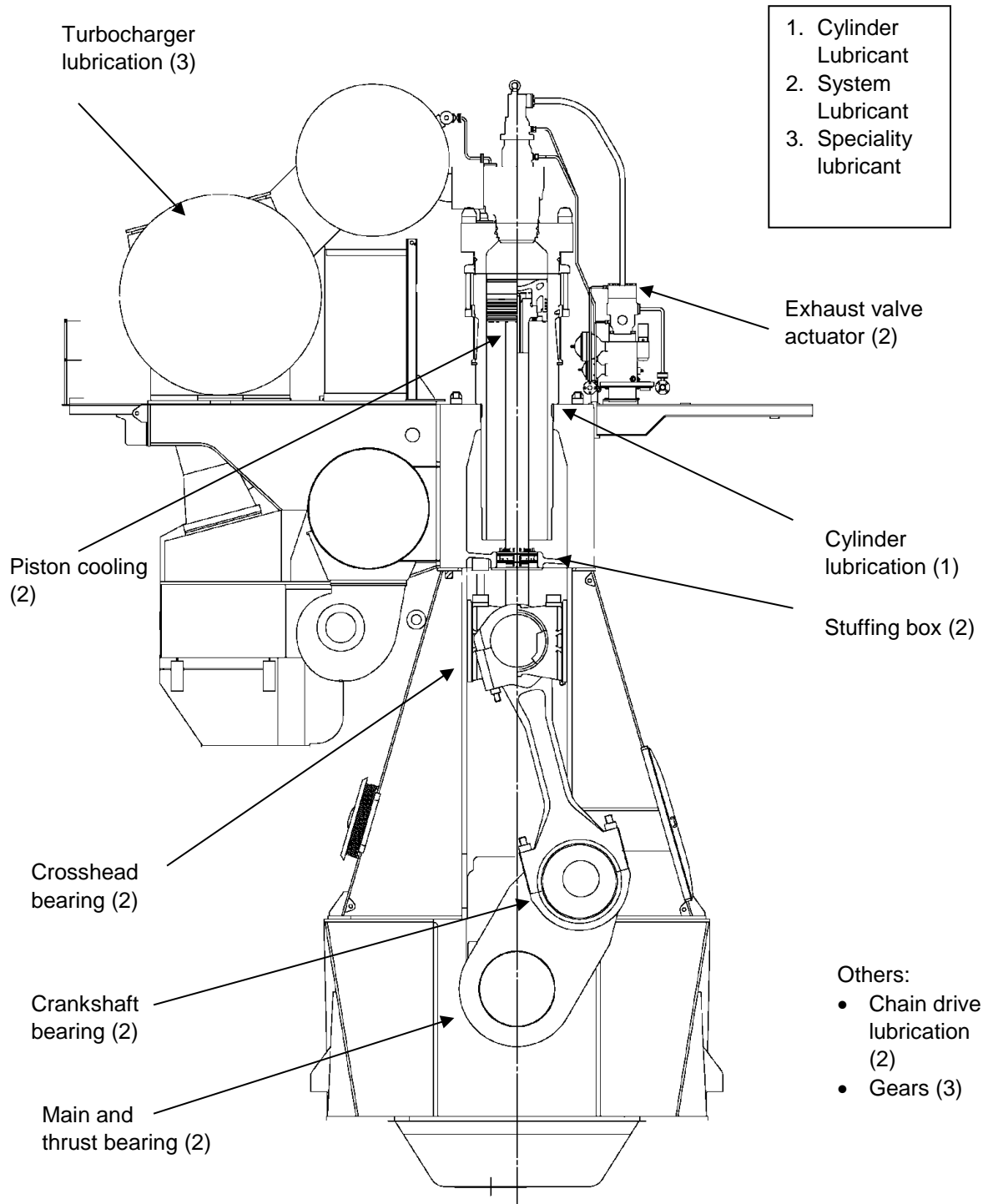
Figure 1: Schematic representation of the two-stroke crosshead diesel engine showing where the different lubricants are used. Combustion chamber is lubricated by cylinder lube oil. All rotating parts
