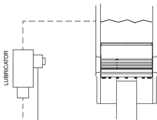
Figure A5: Schematic of cylinder oil supply to oil quills.
