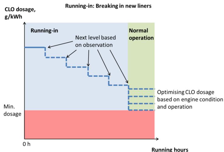
Figure 14: Illustration showing cylinder lube oil feed rate during running-in of new liners. Note that optimizing the feed rate may only be done based on advised decisions e.g. port inspections and drain oil analysis.
