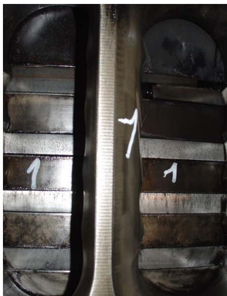
Figure 15: Piston ring microseizures
