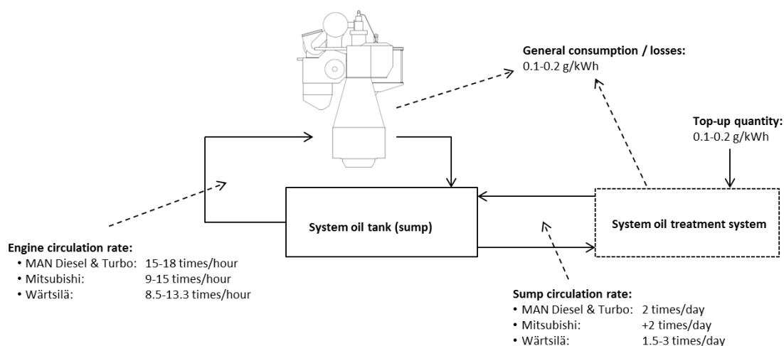
Figure 25: System oil circulation rate and oil consumption
