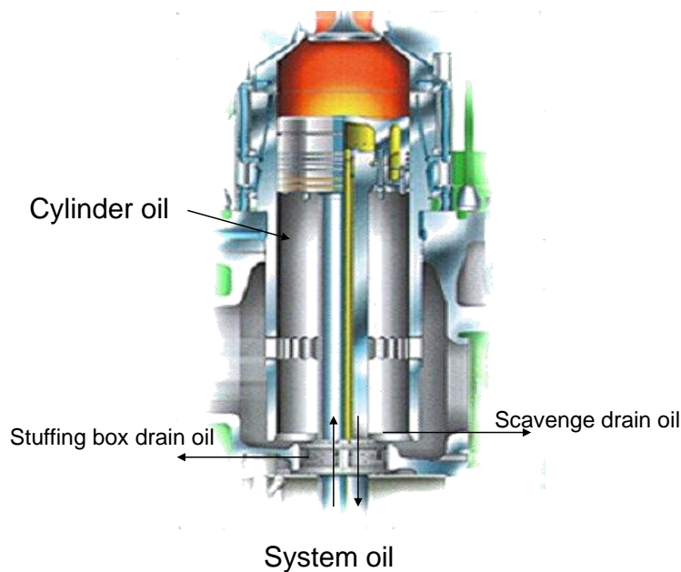
Figure 29: Drain oil location
