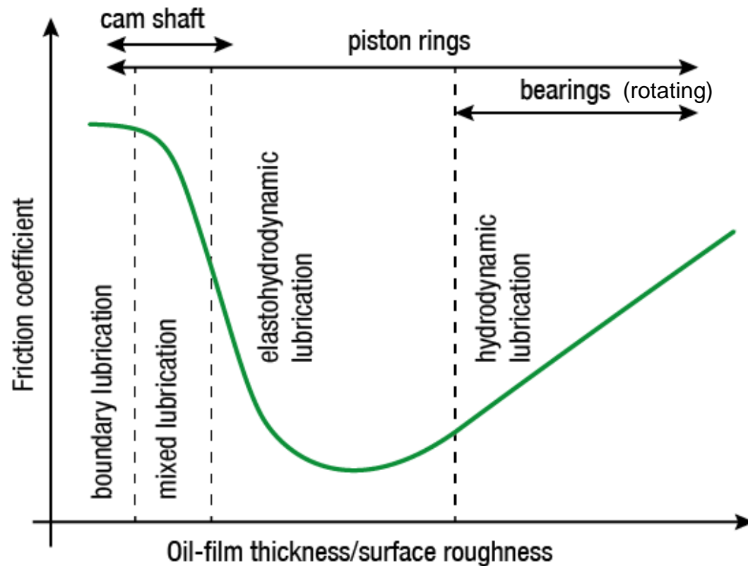
Figure 2: The Stribeck curve. General lubrication conditions for some engine components are shown.
