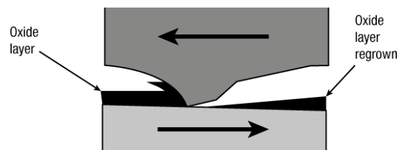
Figure 7: Schematic representation of oxide layer removal – exposing the surface to corrosion
