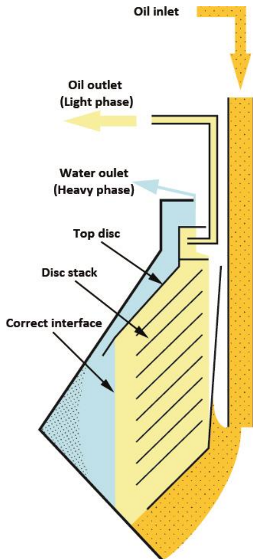
Figure 28: Correct Oil/Water interface position in a purifier
