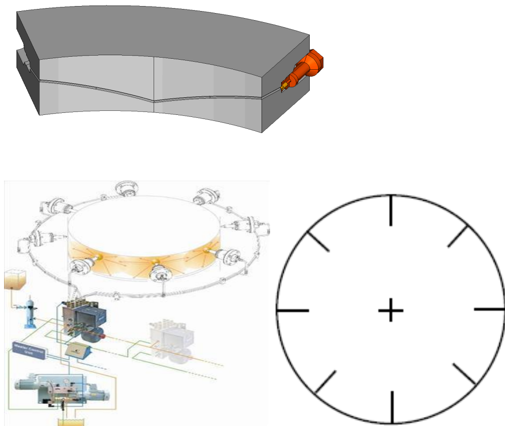
Figure A2: Layout of the CLU4 Pulse Feed and Pulse Jet cylinder oil lubrication system
